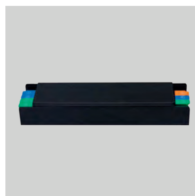
■ ML2649 ■ ML2650 100W 48V 200W 48V 190x48x25mm 205x48x25mm
