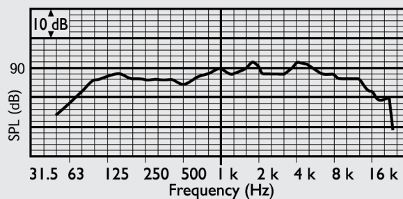
frequency response
