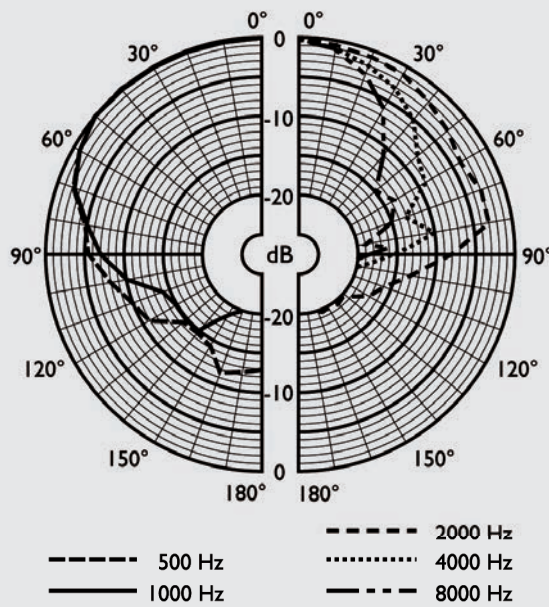
polar diagram
