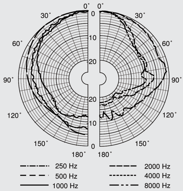
polar diagram
