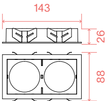
SQUARE - FRAME TWIN (REQUIRED)
