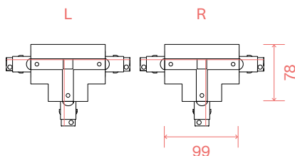
MAIN CONNECTOR T
