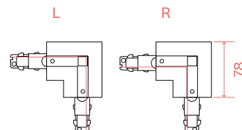
MAIN CONNECTOR CORNER
