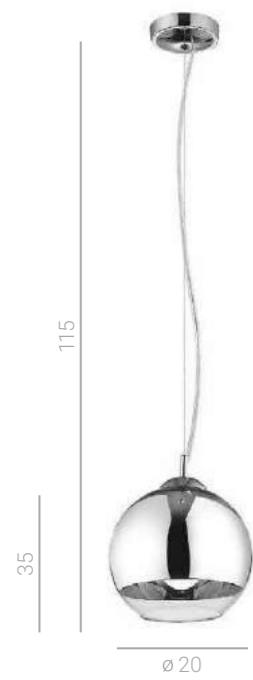
MA04914C-001 ⚡ E27 1x60W
