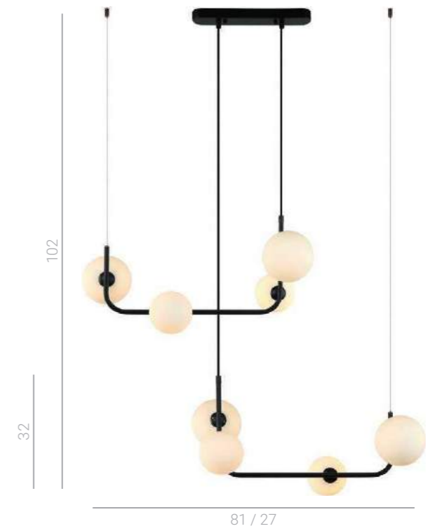
MDM-4123/8 BK ⚡ G9 8x25W
