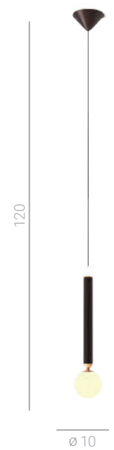
PND-2018109-1 LED 6W 600 lm 3000K
