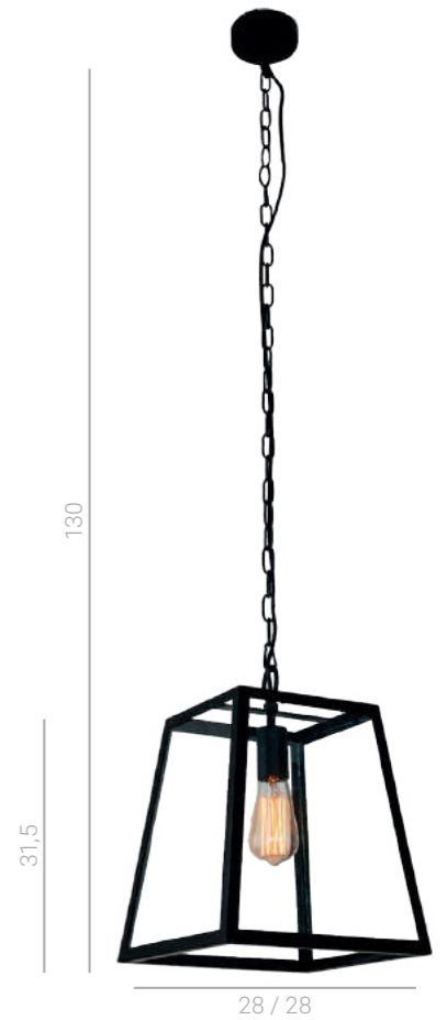
MD-102821-1-B E27 1x60W
