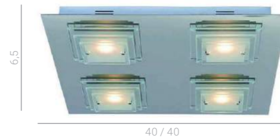
C0509A CLEAR LED 20W 1800 lm 3000K
