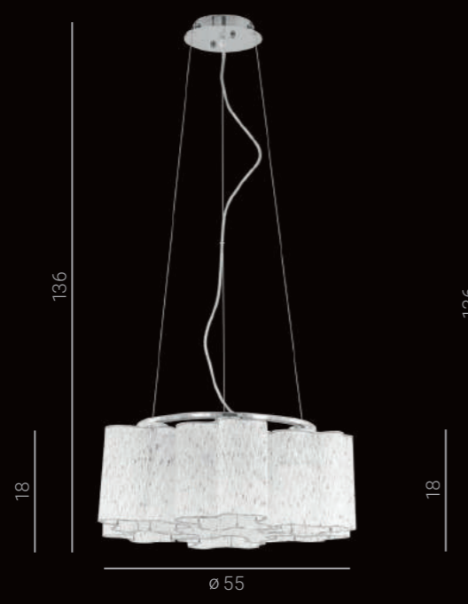
MA03187C-006 ⚡ E27 6x60W
