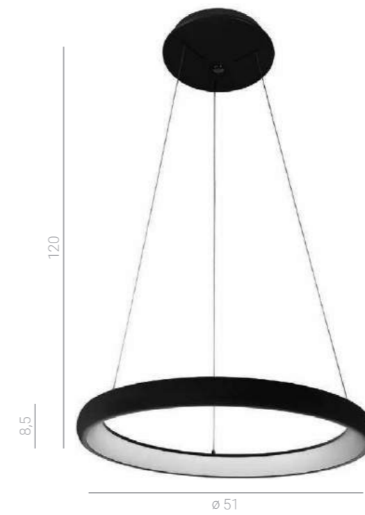
● 5280-840RP-BK-3 ○ 5280-840RP-WH-3 LED 40W 2200 lm 3000K
