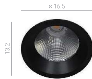
● DG-150C/BK-WW/70 ○ DG-150C/WK-WW/70 LED 34W 3500 lm 3000K IP54
