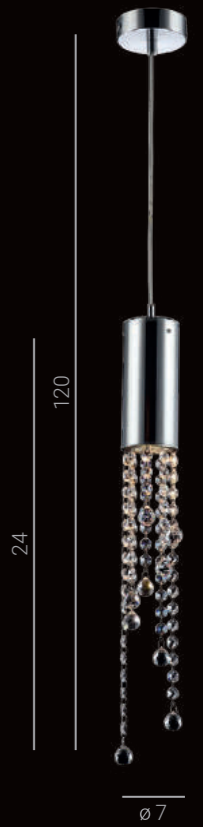
MD93708-1A GU10 1x35W
