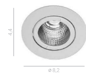
DA-B35D/WK-WW/50 LED 9W 900 lm 3000K IP44
