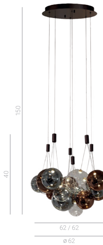
PND-2021955-18 LED 27W 3240 lm 3000K
