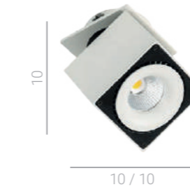
SL7562/28W 3000K WH+BL SL7562/28W 4000K WH+BL LED 28W 2350 lm 3000K / 4000K
