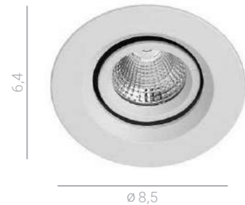
DA-401C/WK-WW/50 LED 13W 1300 lm 3000K IP44
