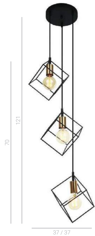
MDM-4244/3 BK+BRO ⚡ E27 3x40W
