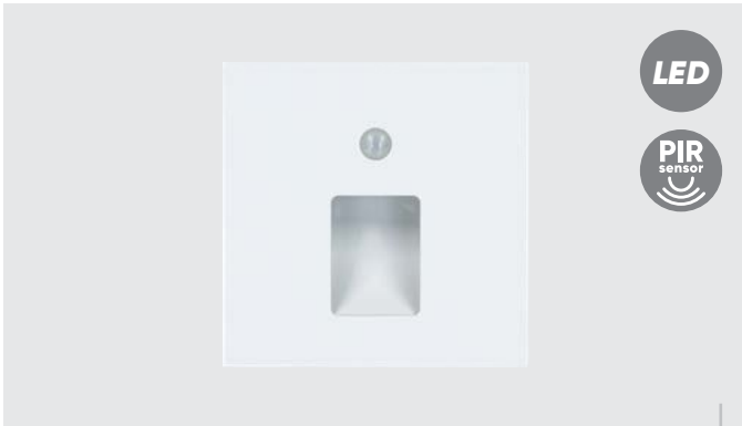
71420 Step light Vix S ↔87mm ↓87mm ↗35mm
