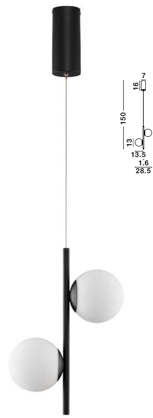
NUVOLE - 9061436 Sandy Black Aluminium & Opal Glass LED 16 Watt 220 Volt 800Lm 3000K IP20 L: 28.5 W: 13 H: 150 cm
