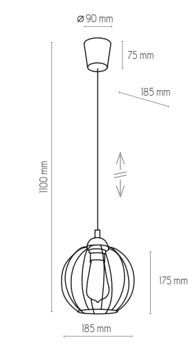
1644 | GALAXY | 1 x E27, max 60W | DM 13
