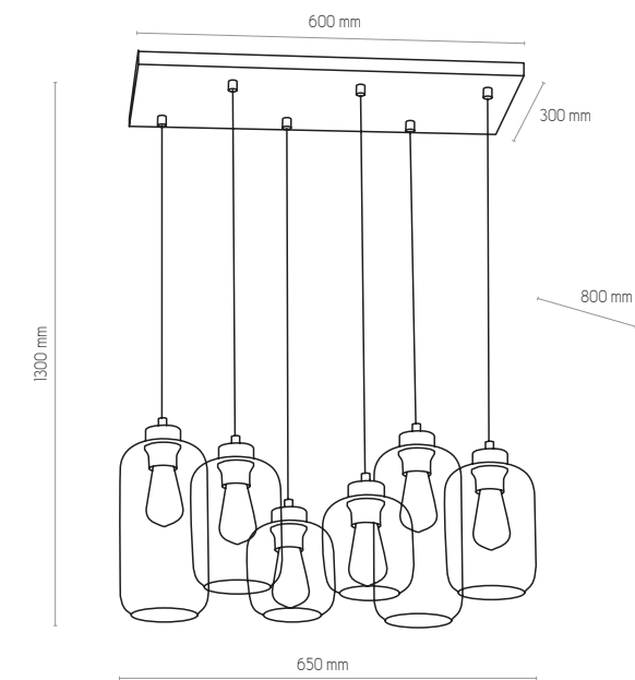
3359 | MARCO SILVER | 5 x E27, max 60W
