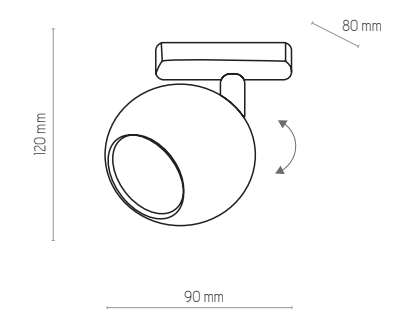
4040, 4041 | TRACER | 1 x GU10, max 50W
