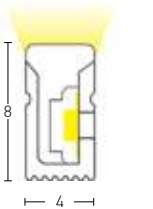
End Cap Code ECLS08-09
