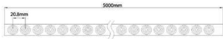
-FLEXIBLE WALL WASHER 3D 24V 24W/m with OPTICS 20° x 35°
